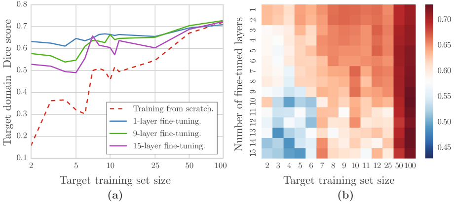
Fig. 2. (a) The comparison of Dice scores on the target domain with and without transfer learning. A logarithmic scale is used on the x axis. (b) Given a deep CNN with d = 15 layers, transfer learning was performed by freezing the i initial layers and fine-tuning the last d - i layers. The Dice scores on the test set are illustrated with the color-coded heatmap. On the map, the number of fine-tuned layers are shown horizontally, whereas the target domain training set size is shown vertically.
